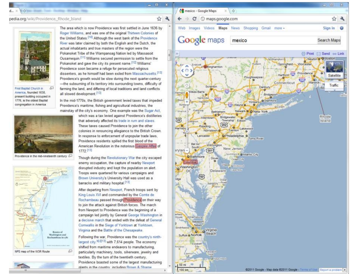
Frame-Based Highlighting
