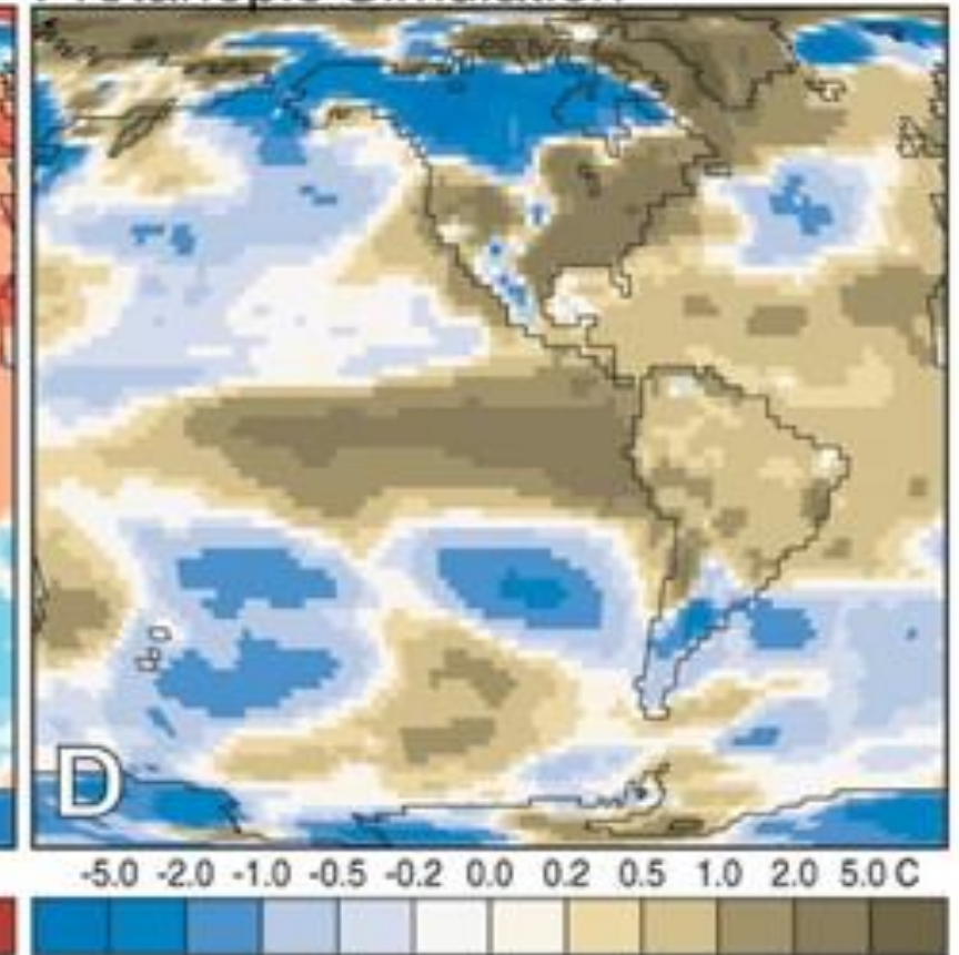
Protanopic Simulation
