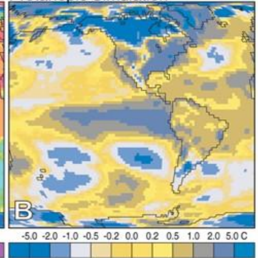
Protanopic Simulation
