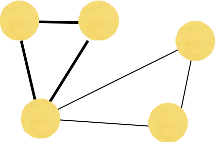
A cycle
