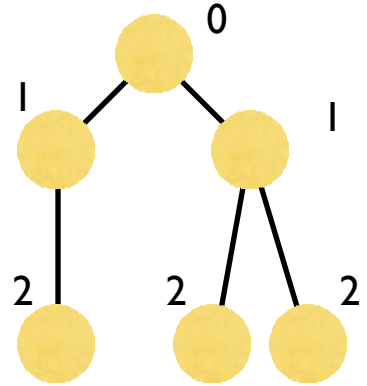
Node depths
