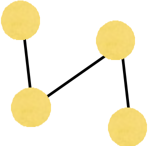
An acyclic graph
