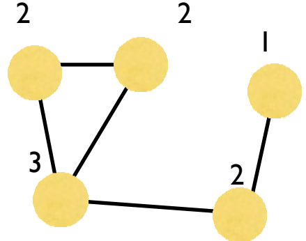
Node degrees
